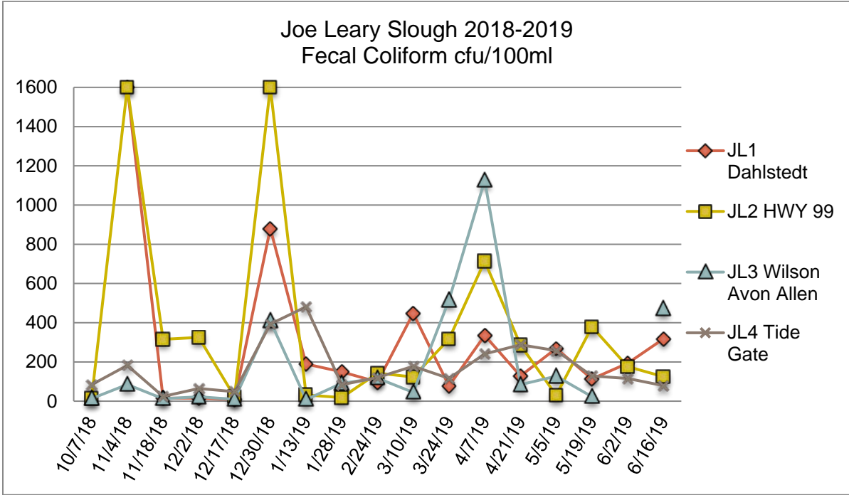
Figure 64. Joe Leary Slough Fecal Coliform: 2018-2019
