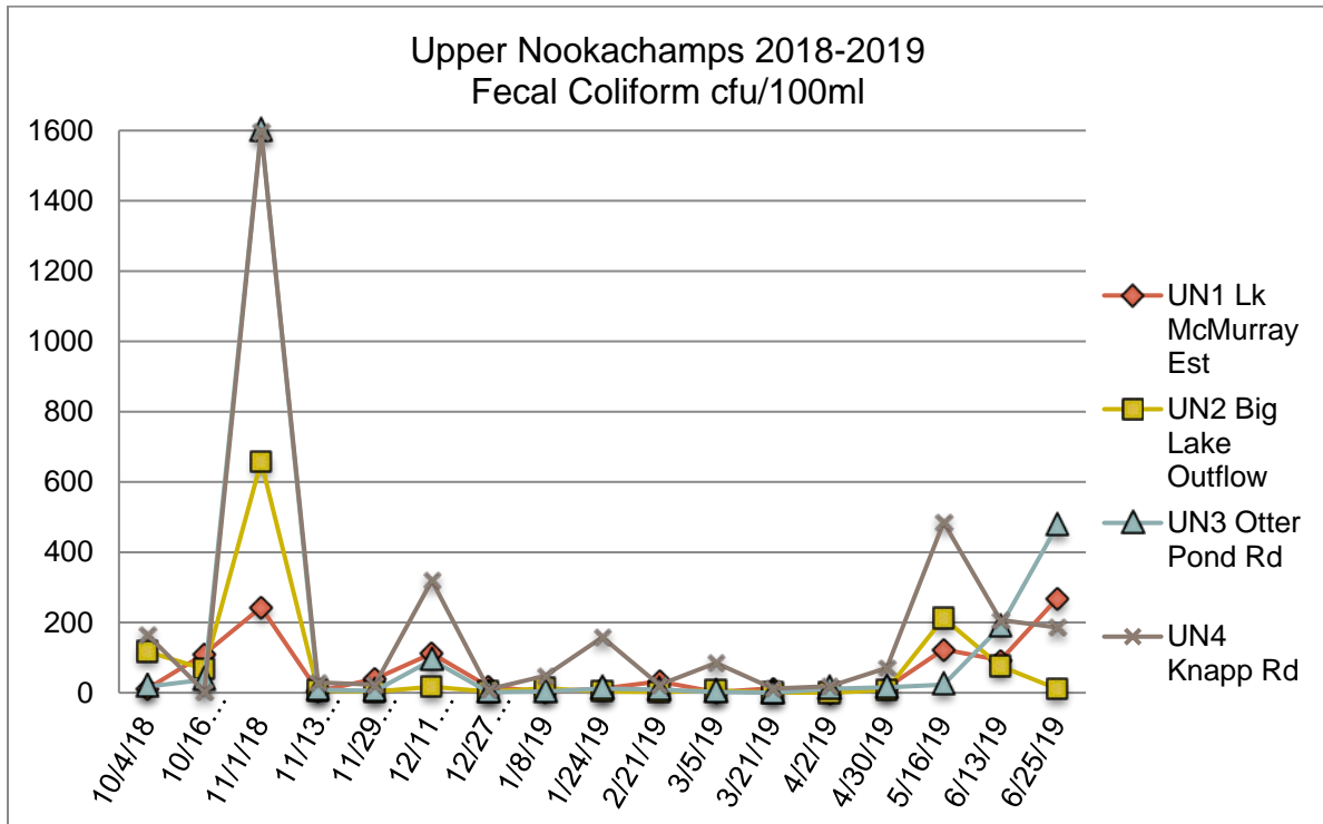
Figure 32. Upper Nookachamps Fecal Coliform: 2018-2019
