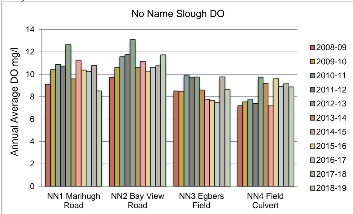
Figure 43. No Name Slough DO: Eleven-year comparison
