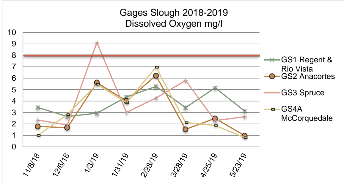
Figure 90. Gages Slough DO: 2018-2019
