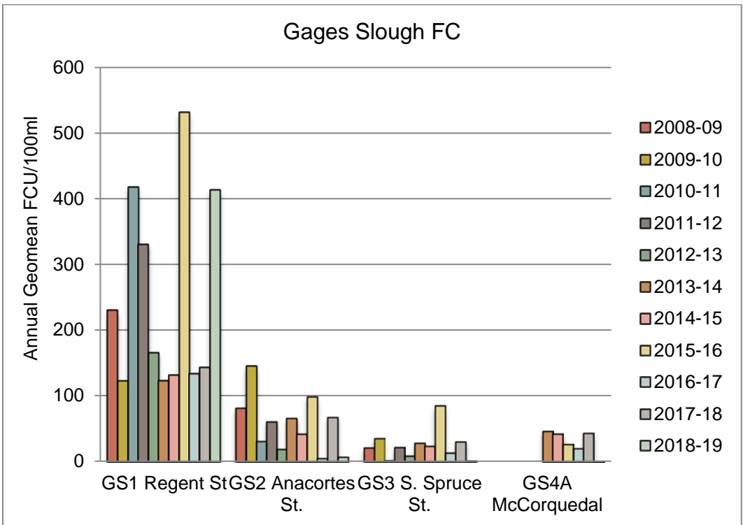
Figure 97. Gages Slough Fecal Coliform: Eleven-year comparison
