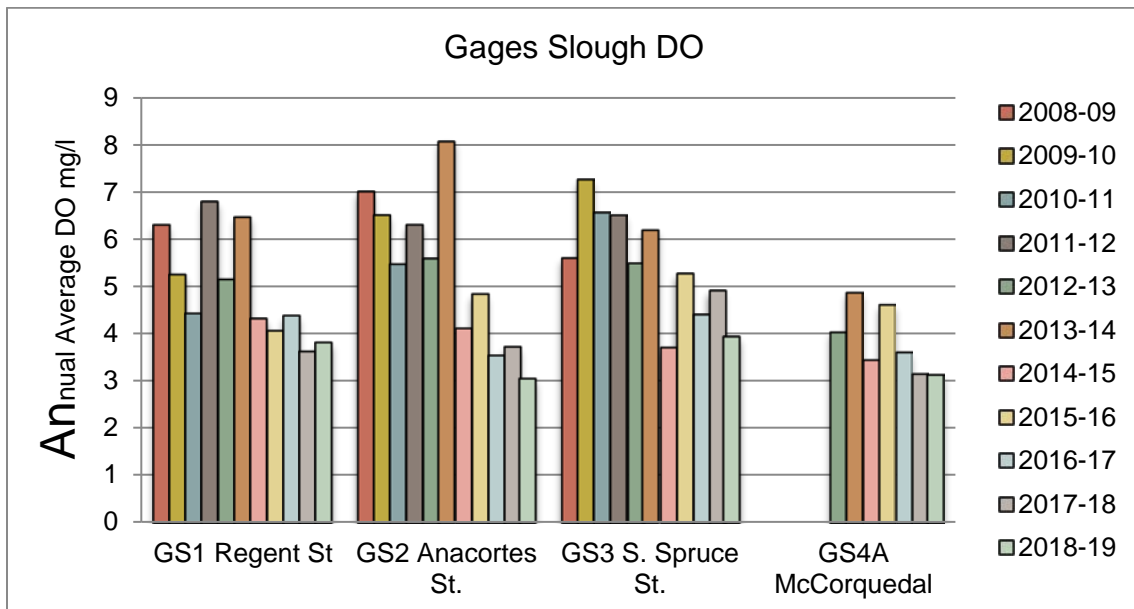
Figure 91. Gages Slough DO: Eleven-year comparison
